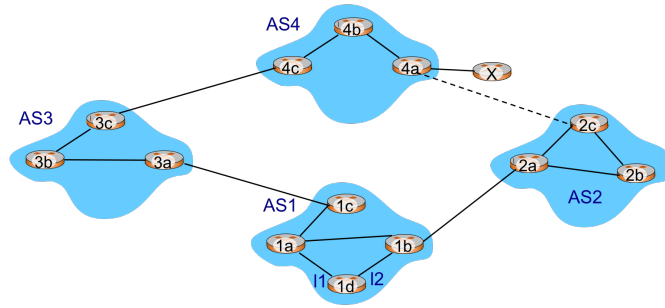
Figure 4: Network topology
