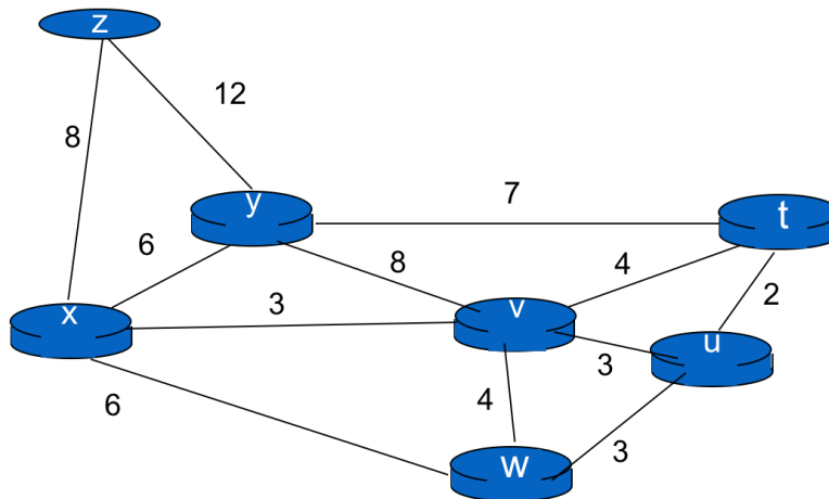
Figure 3: Network 1.
