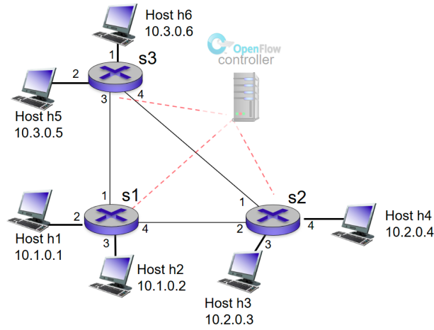
Figure 2: OpenFlow match-plus-action network with three packet switches, 6 host, and an OpenFlow controller
